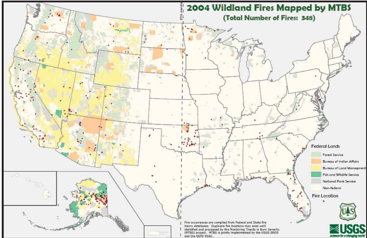
Figure 5. Location of 2004 wildland fires mapped by MTBS.
