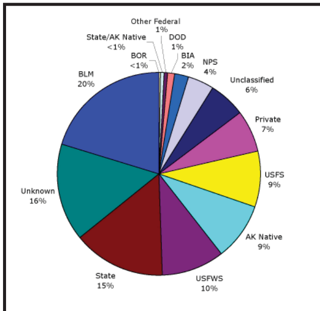
Figure 8. Percent of the total burned area in 2004 by government administration.
