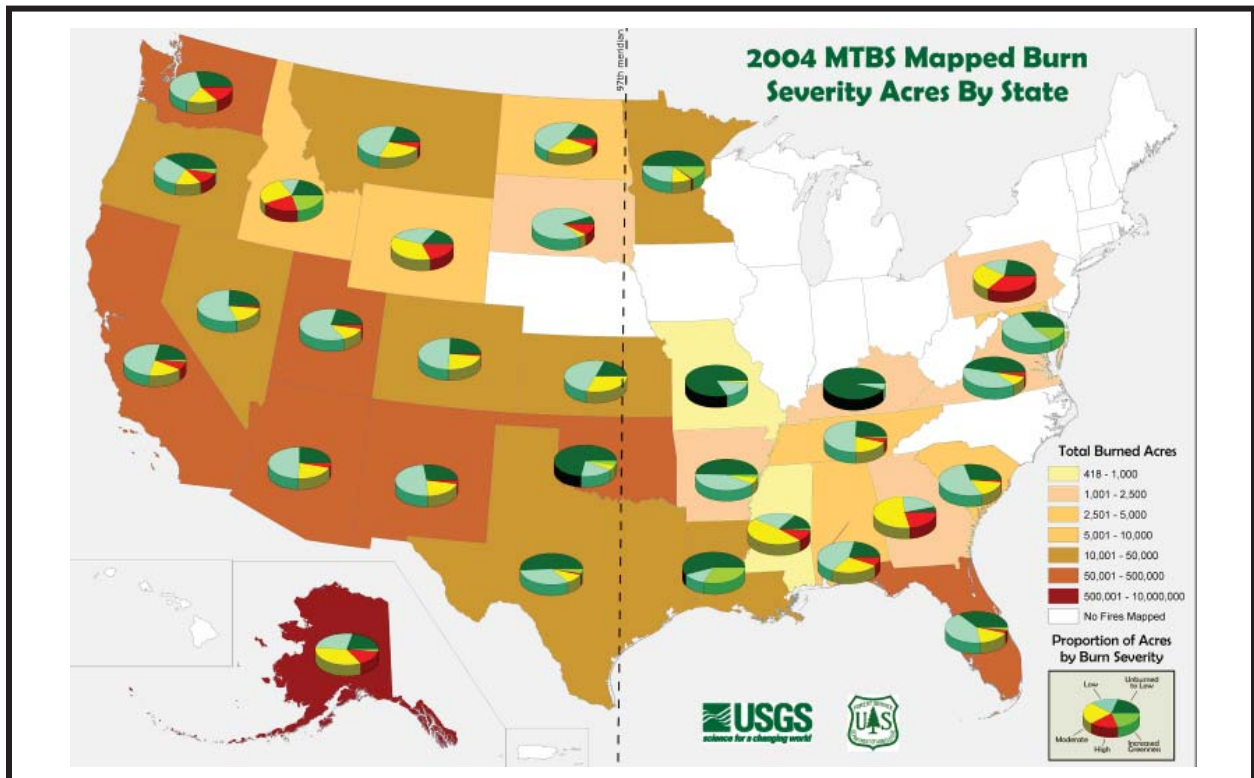
Figure 11. The states most affected by fire in 2004 (total acres burned).
